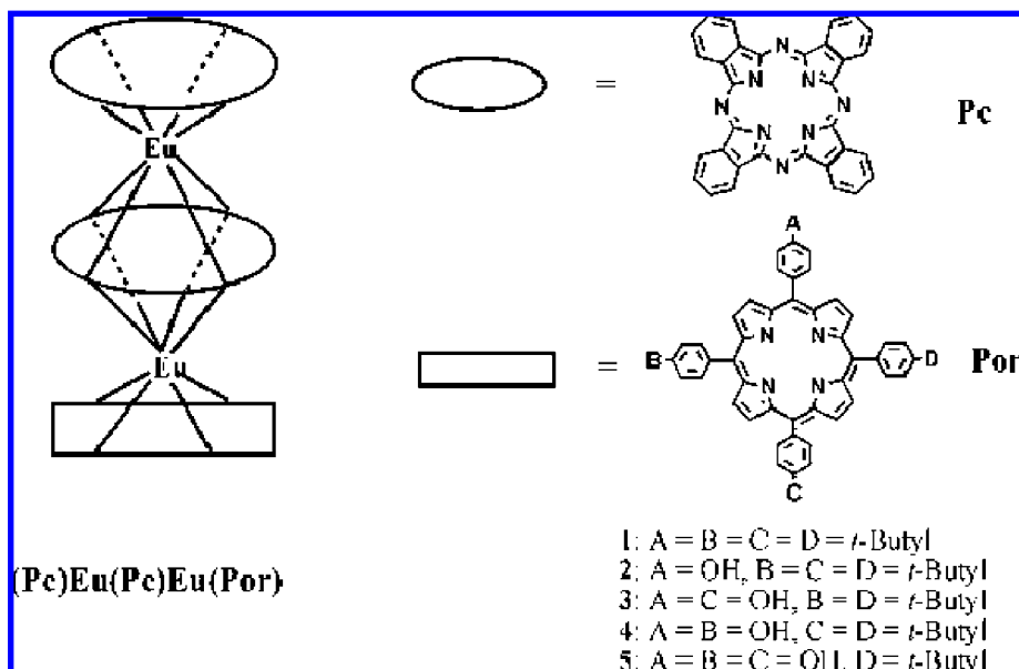
Figure 1. Schematic molecular structures of the mixed (phthalocyaninato)(porphyrinato) europium triple-decker complexes 1–5.
